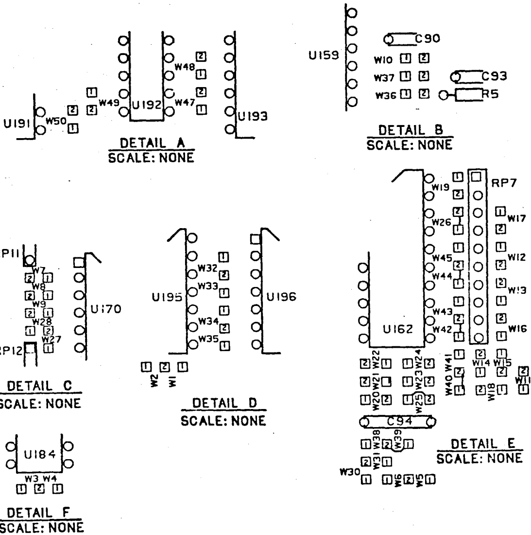
FIGURE 3-1B NS235 JUMPER DRAWING
